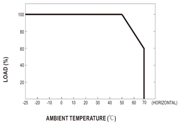
■Drating Curve
