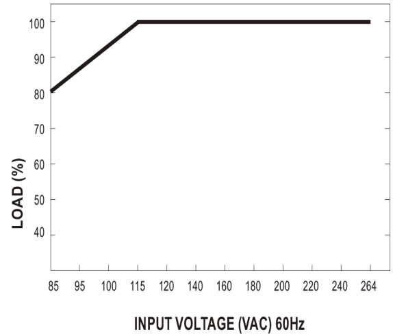
■Static characteristic
