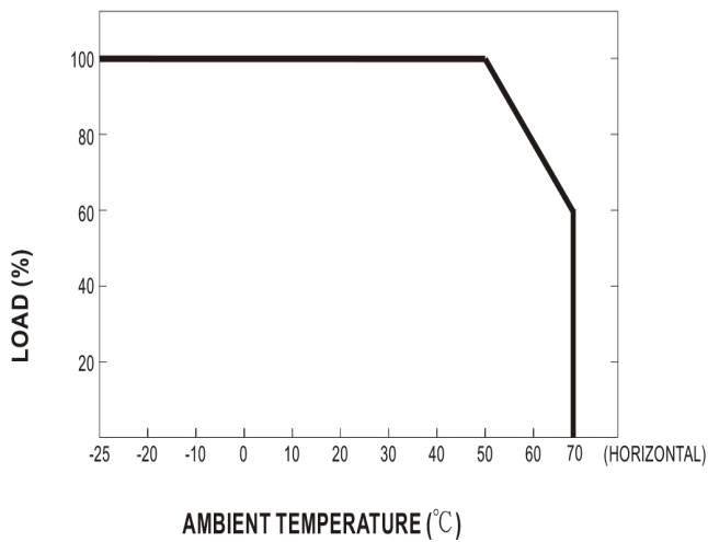
■Drating Curve
