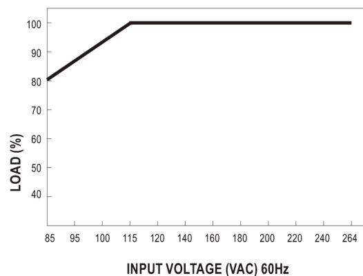
■Static characteristic
