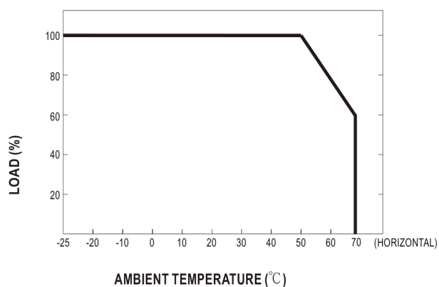
■Drating Curve
