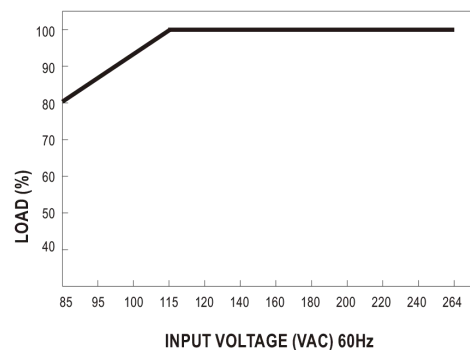
■ Static Characteristics
