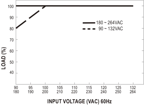
Static Characteristics
