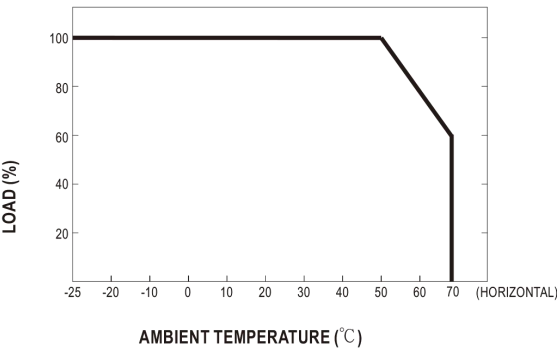
Derating Curve
