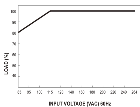
■ Static Characteristics
