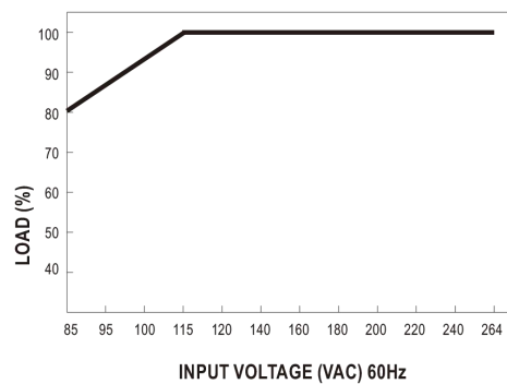
■ Static Characteristics
